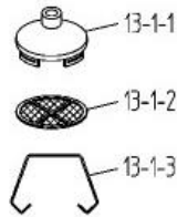
⑬-1 塗料吸込濾過器 Fluid intake filter
